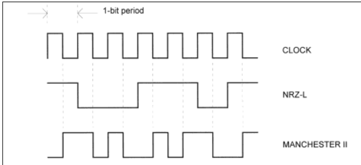
Figure 4-4. A Manchester II Encoded Sequence
